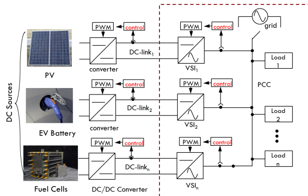
Fig. 1: A schematic of a microgrid. An array of DC power sources provide power at the respective DC-links, where the voltage is regulated by DC/DC converters. A network of parallel inverters that connect to the DC-links convert the total current from the sources at the regulated voltage to alternating current (AC) at its output to satisfy the power demands of the AC loads.
