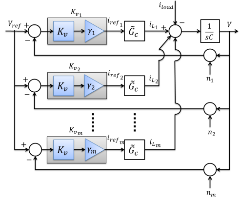
Fig. 3: Proposed decentralized framework with smart choices of controller parameters. The inner-current controllers K_{c_k} are chosen such that the inner-shaped plant mimics \tilde{G}_c(s) shown in the discussion after Eq. (8). The outer-loop controllers are scalar multiples of the nominal outer-loop controller K_v ; the scalars \gamma_k govern the power-sharing requirements in a microgrid setup.
