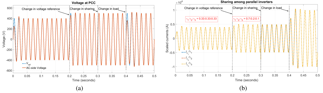
Fig. 5: Results for a network of three parallel inverters for (a) Voltage regulation (b) Power sharing.
