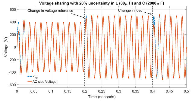
Fig. 4: Voltage regulation using the proposed controllers for 20% uncertainty in L and C values.
