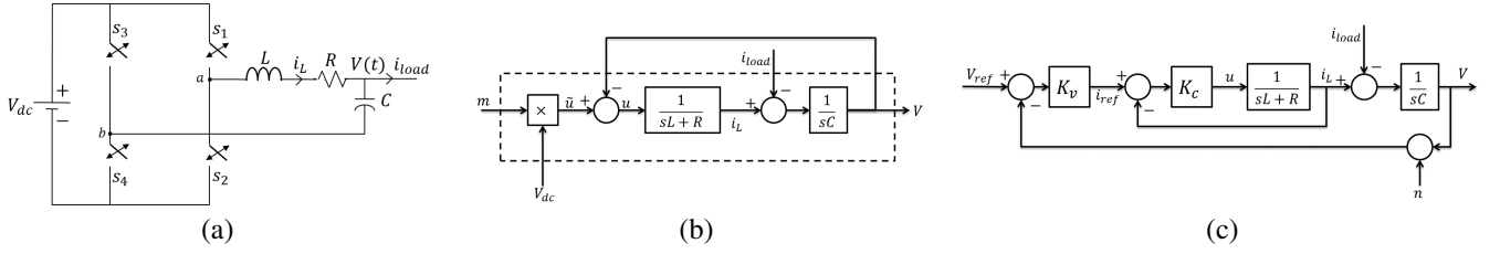
Fig. 2: (a) Circuit representing a full-bridge inverter. The AC-side current is given by i_{load} . The switches s_1, s_2, s_3 and s_4 control the AC-side voltage V(t) . (b) Associated control model of the full-bridge inverter. (c) Inner-outer control architecture of a full-bridge inverter.
